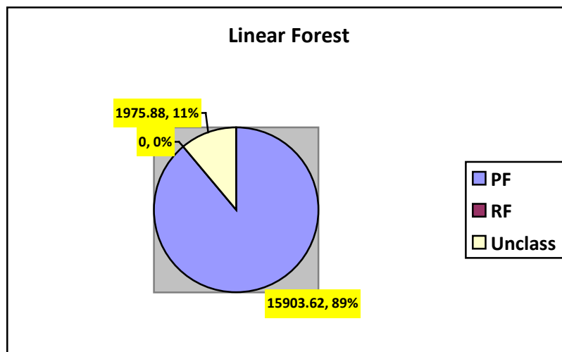
Figure 3: Linear Forests
